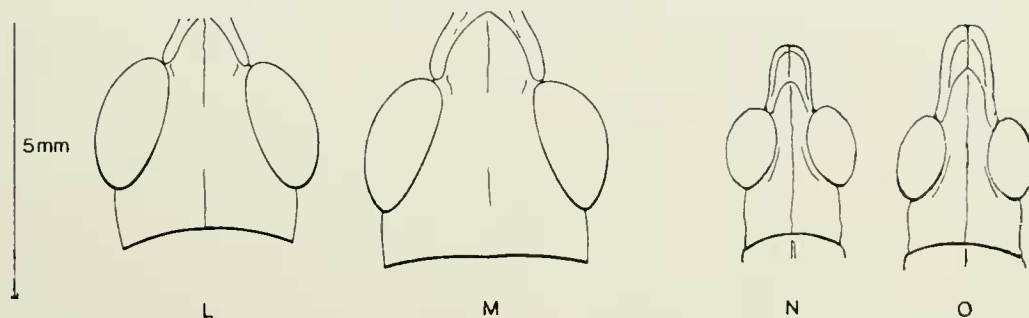
Figure 1. Dorsal view of heads of Ichthiacris spp. A, B, I. (I.) rehni , ♂, ♀; C, I. (I.) spinifera , ♂, holotype; D, I. (I.) spinifera , ♀ allotype; E, F, I. (Atyphacris) elongata , ♂, ♀; G, H, I. (A.) costulata , ♂, ♀; I, J, I. (A.) californica , ♂, ♀; K, I. (A.) celata , ♂; L, M, I. (A.) aptera , ♂, holotype; O, I. (I.) parva , ♀; N, I. (I.) parva , ♂, ♀ (last-instar juv.).
